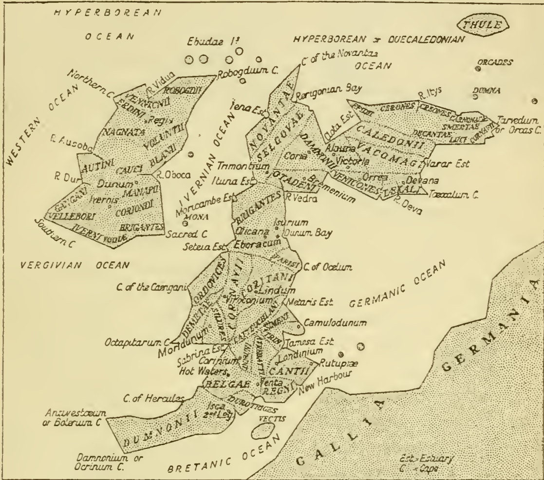
FIG. 28. Map of British Isles reconstructed by plotting out the fixed points given by Ptolemy and joining them together by straight lines.
